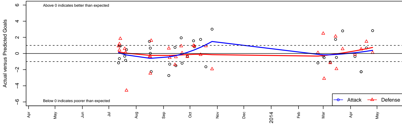
Westside Timbers Mundial B02 Dots are actual minus expected GF (blue circles) and GA (red triangles). Blue line is smoothed change in attack strength. Red is smoothed change in defense strength.
